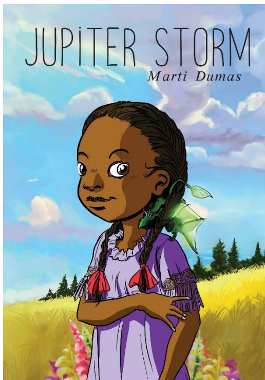
Jupiter Storm-High Resolution
